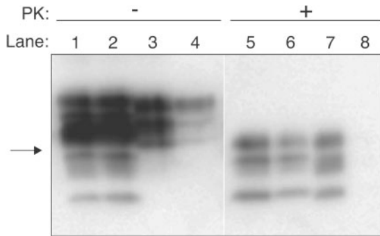
FIG. 1. Deposition of the abnormal isoform of the prion protein, PrP res , in the brain of squirrel monkeys inoculated with chronic wasting disease. Western blot analysis of 250- \mu g tissue equivalents of brain homogenates digested with proteinase K or not digested with proteinase K was performed. The brain homogenates were from a CWD-infected squirrel monkey that was sacrificed at 34 months (lanes 1 and 5) or at 31 months postinfection (lanes 2 and 6), a CWD-infected elk (lanes 3 and 7), and an uninfected mouse (lanes 4 and 8). The arrow indicates the location of the 29-kDa molecular mass marker.
